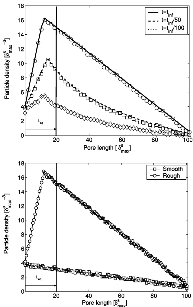
FIG. 9. Molecular density profile along a pore. (a) Density profile for a rough pore [ \xi=(13/9)^2 ] after different clock times ( t_{inf} is a long time, when steady state is reached). (b) Comparison of the density profiles in a smooth and in a rough pore.
